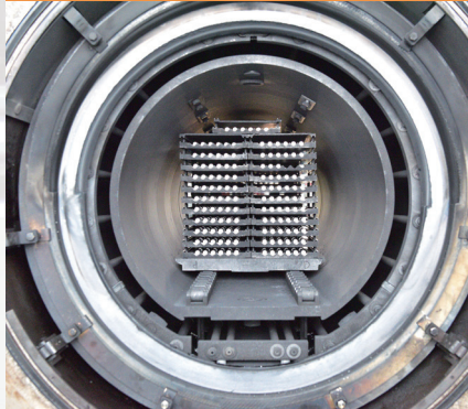
Sintering
